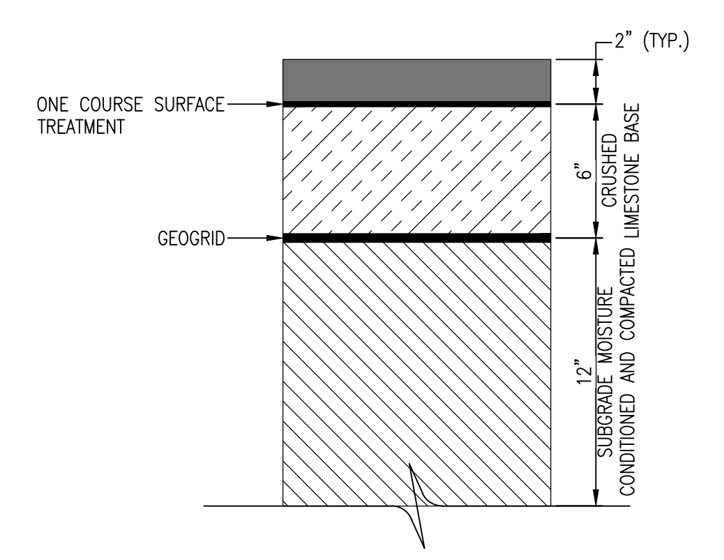
PRELIMINARY PAVEMENT SECTION
