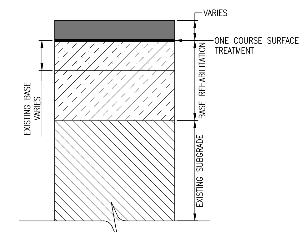
PRELIMINARY PAVEMENT SECTION
