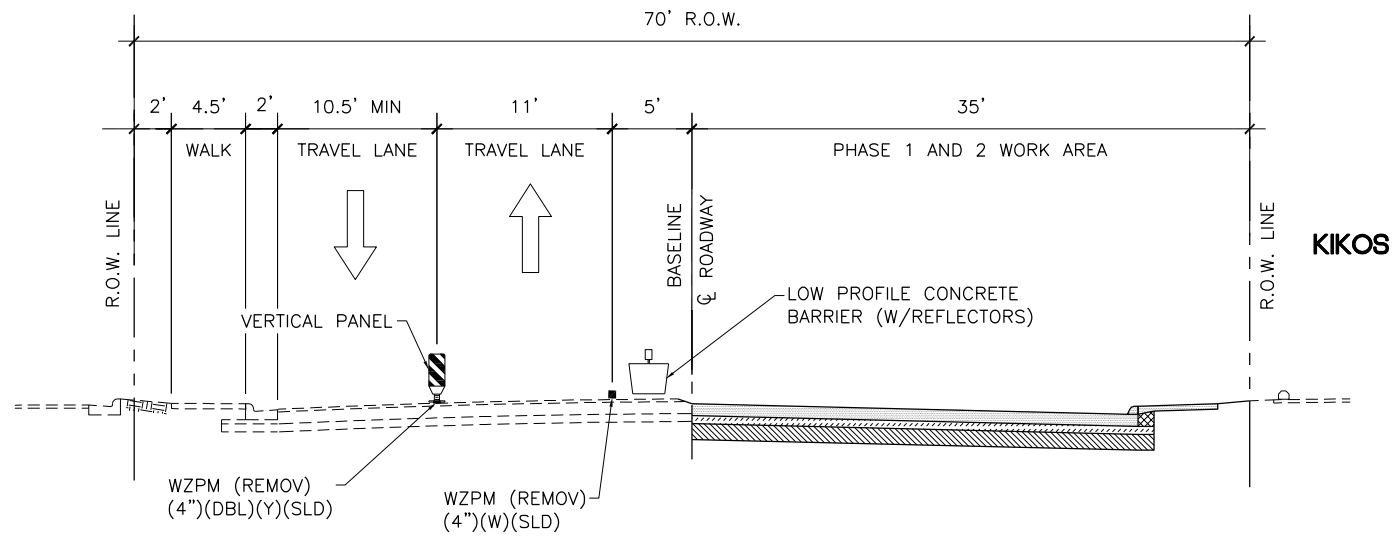
PHASE 1 AND PHASE 2 TRAFFIC CONTROL SECTION
