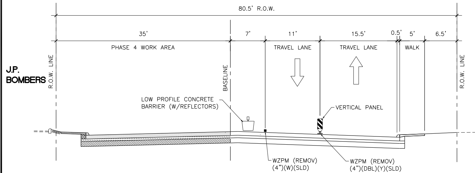
PHASE 4 TRAFFIC CONTROL SECTION
