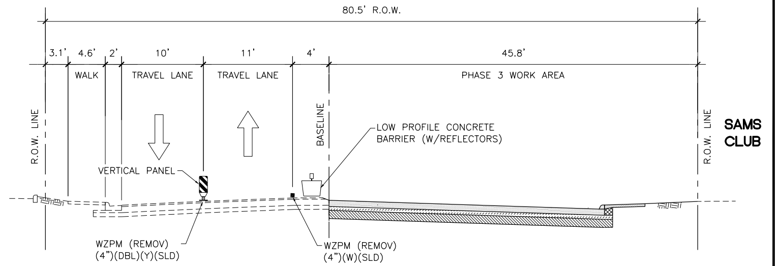
PHASE 3 TRAFFIC CONTROL SECTION
