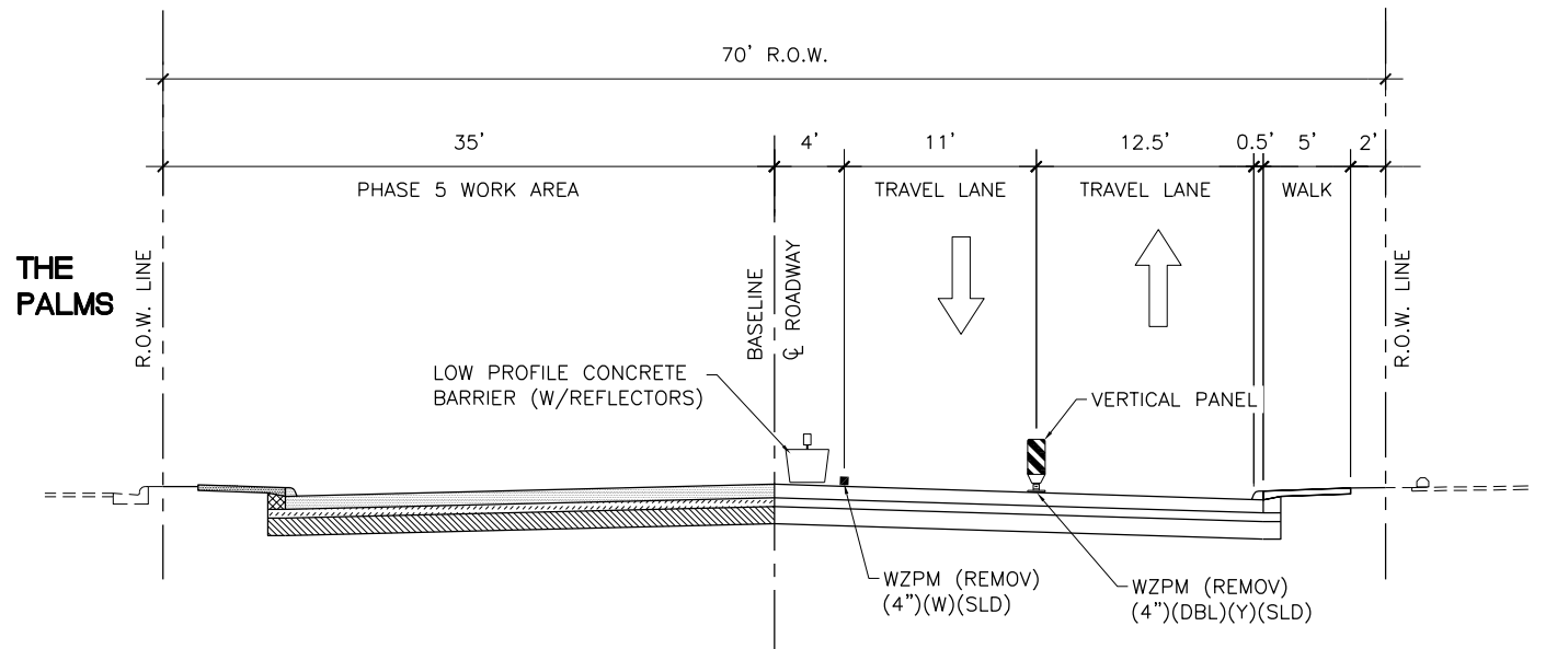
PHASE 5 TRAFFIC CONTROL SECTION
